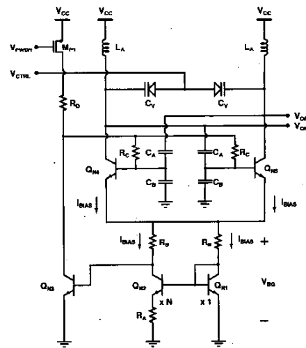
Fig. 1. VCO schematic (VCO embedded in Widlar-bandgap).
