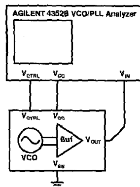
Fig. 5. Measurement setup.
