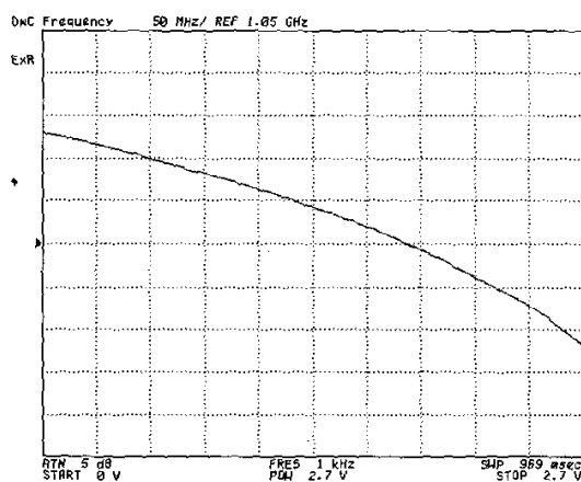
Fig. 8. Tuning Characteristics.
