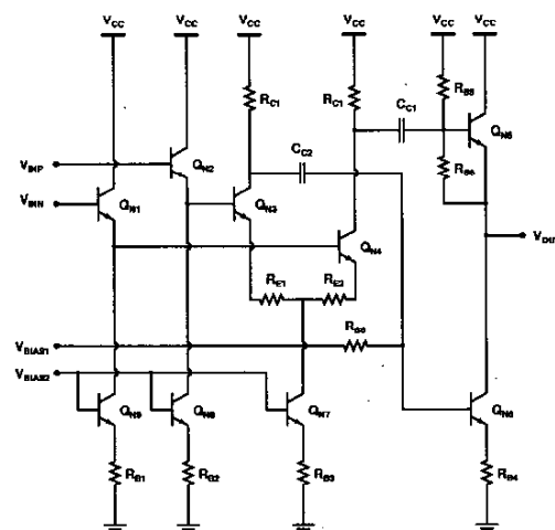
Fig. 3. Output buffer schematic.
