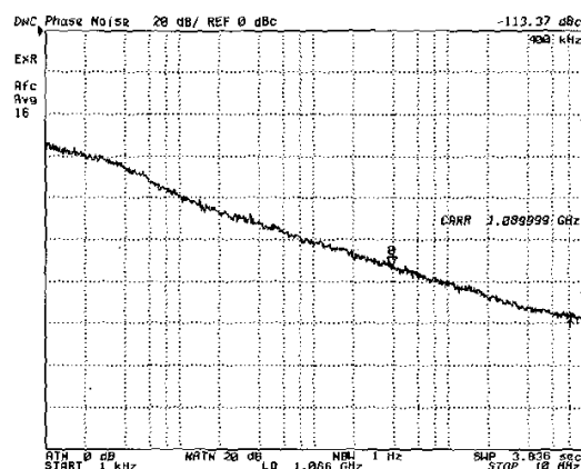
Fig. 7. Phase noise.
